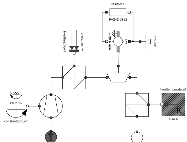
Figure 2: Joule-Brayton cycle using ThermoSimT.
