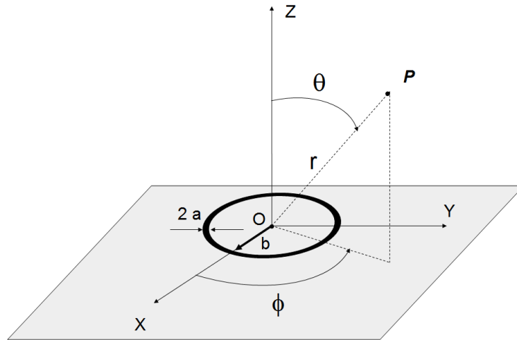
Figure 1: Cartesian (X, Y, Z) and polar (r, \phi, \theta) coordinates of a point P . The horizontal circle of radius b is a single conduction loop of diameter 2a .
