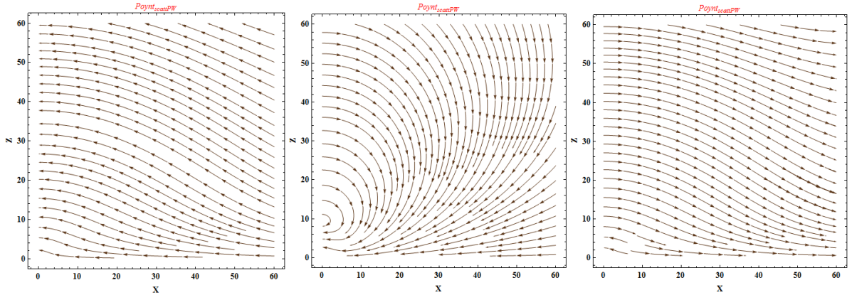
Figure 5: Scattered Poynting-vector fluxes at f < f_{res} (left), f = f_{res} (center) and f > f_{res} (right).
