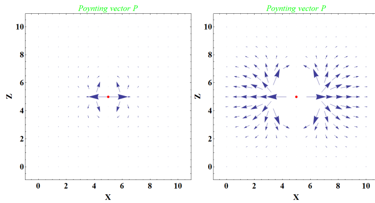
Figure 4: Poynting vector field (power flux) in the XZ -plane under the same conditions as in figures 2 and 3. Arrow lengths are proportional to the power flux intensities (Poynting norm).
