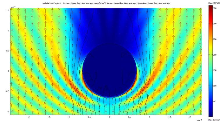
Figure 7: Strong absorption of an EM wave of wavelength \lambda = 4 [nm] by a spherical particle with a diameter of 15 [nm]: Black full lines represent Poynting flux, with norm indicated by the background colours. Arrows represent the Poynting vectors.
