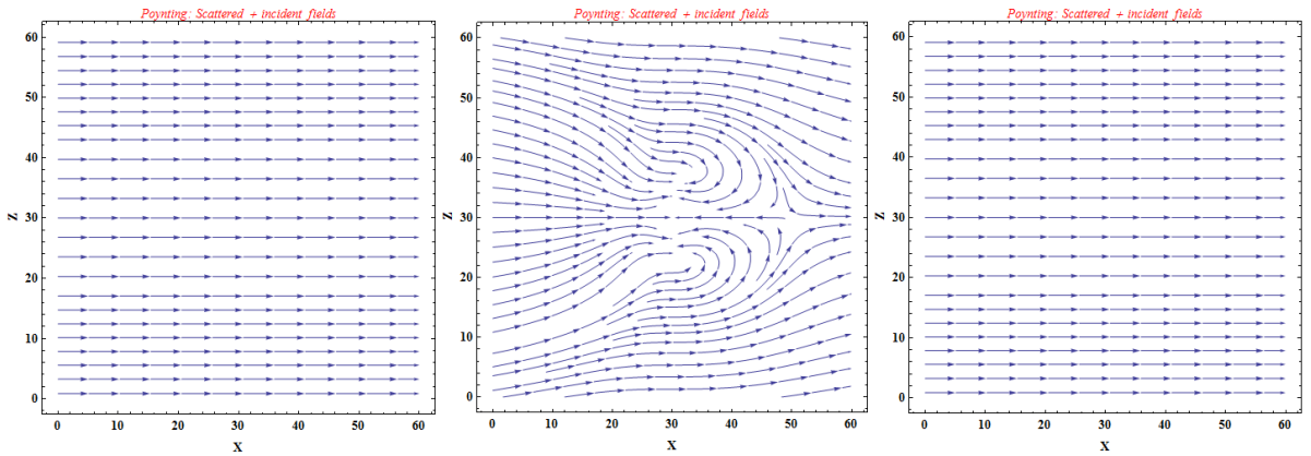
Figure 6: Power flux lines in the XZ -plane at frequencies 0.90 f_{res} (left), f_{res} (center) and 1.10 f_{res} (right). The field arrows are not drawn to scale, they only show the local field directions. Notice that the solenoid's centre is now at x_0 = z_0 = 30 [m].
