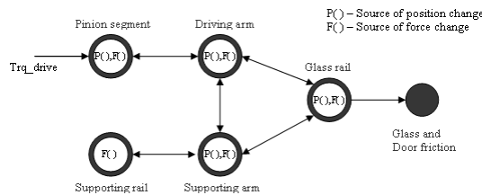
Figure 6: Diagram of cross arm window regulator
