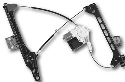
Figure 2: Double rail guided cable driven window regulator
