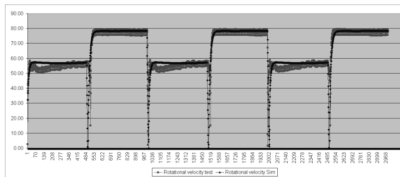
Figure 8: comparison between simulation result and practical measurement
