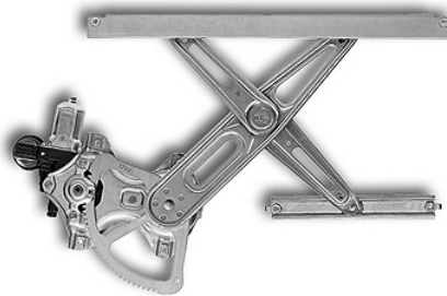
Figure 1: Cross arm window regulator
