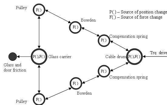
Figure 5: Diagram of single rail window regulator
